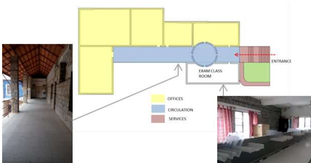
BLOCK B- SECOND FLOOR- TRAINING BLOCK
